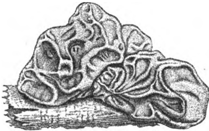
FIG. 326. — Tremella mesenterica ; \times \frac{1}{2} . The body is gelatinous, and the basidia form on the surface. (After Tulasne, from Bennett and Murray, Cryptogamic Botany .)
